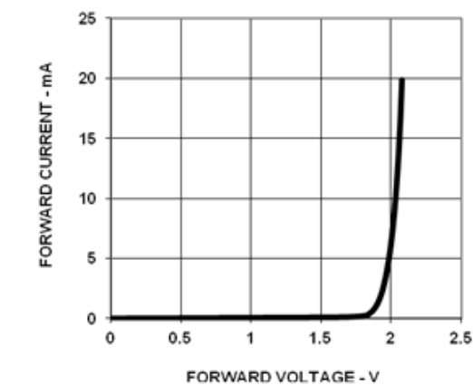
Figure 13: Forward Voltage vs. Current (DP)
