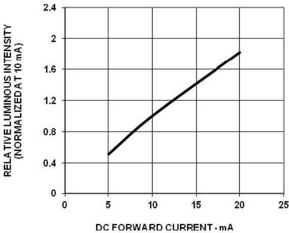
Figure 3: Relative Luminous Intensity vs. Forward Current
