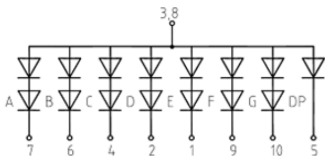
Common Anode
