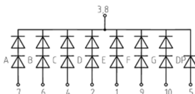
Common Cathode
