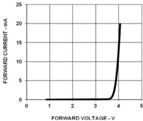
Figure 12: Forward Voltage vs. Current (Segment)
