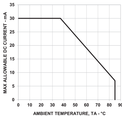
Figure 16: Maximum Forward Current vs. Ambient Temperature
