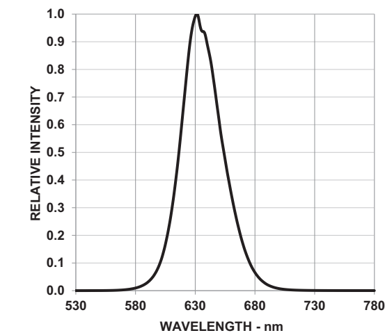
Figure 5: Relative Intensity vs. Wavelength
