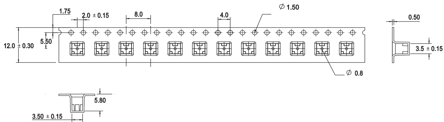
Figure 11: Carrier Tape Dimensions
