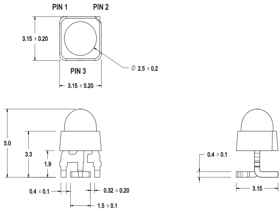
Figure 1: Package Drawing
