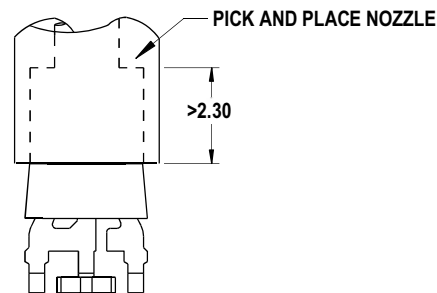
Figure 14: Recommended Nozzle Dimension
