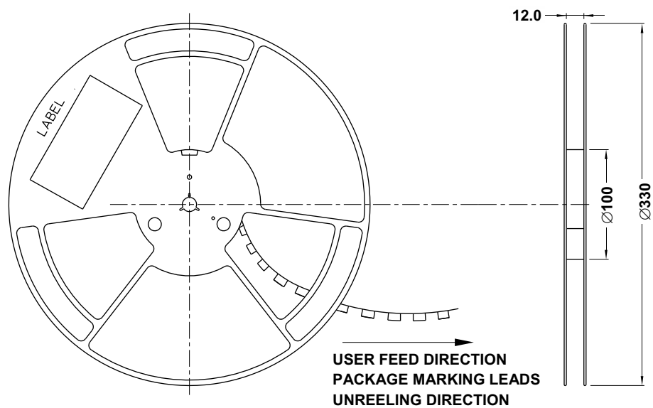
Figure 12: Reel Dimensions
