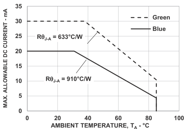
Figure 9: Maximum Forward Current vs. Ambient Temperature. Derate based on T_{J\text{ MAX}} = 110^{\circ}\text{C} (Green), T_{J\text{ MAX}} = 100^{\circ}\text{C} (Blue).
