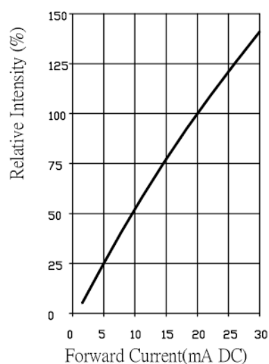
Relative Intensity vs. Forward Current
