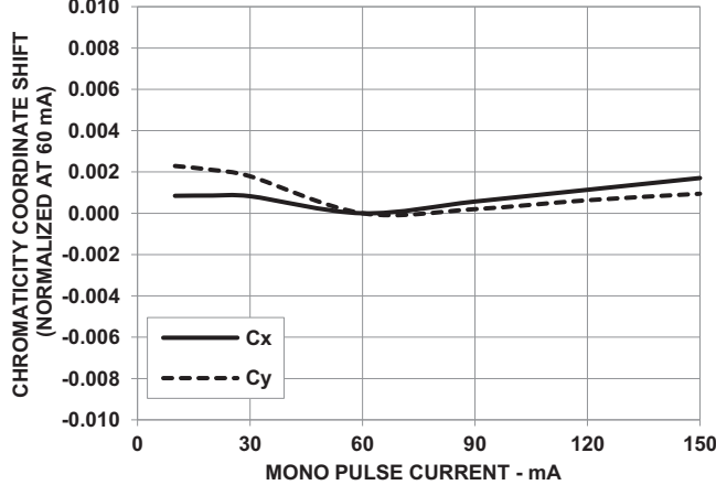
Figure 7: Chromaticity Coordinate Shift vs. Mono Pulse Current for 4000K
