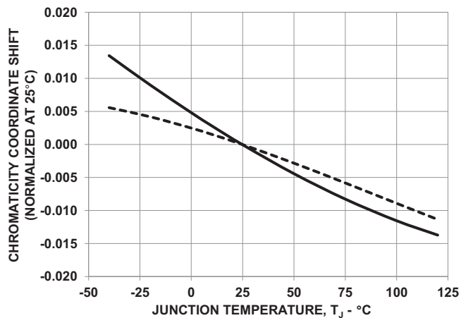
Figure 12: Chromaticity Coordinate Shift vs. Junction Temperature for 6500K
