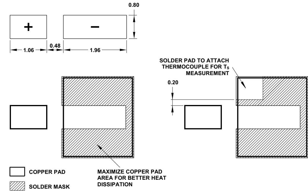
Figure 15: Recommended Soldering Land Pattern
