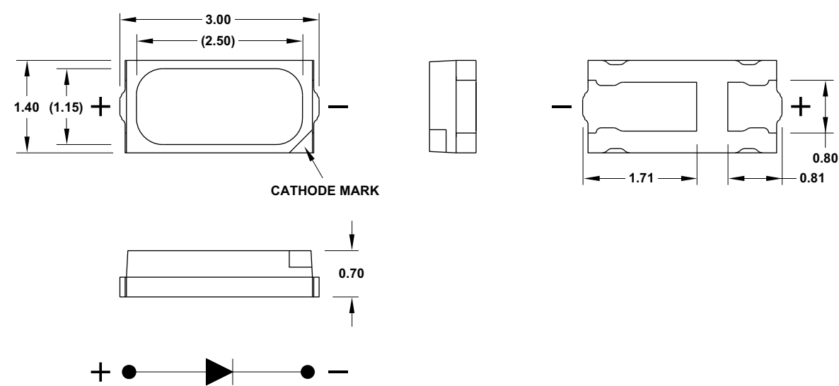
Figure 1: Package Drawing
