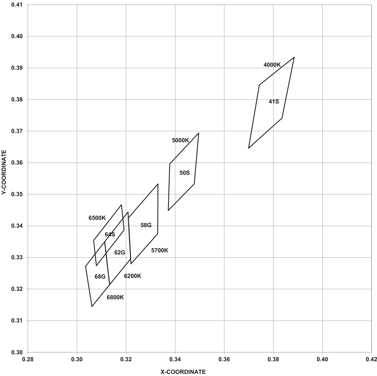
Figure 2: Chromaticity Diagram
