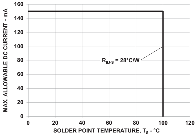
Figure 14: Maximum Forward Current vs. Solder Point Temperature
