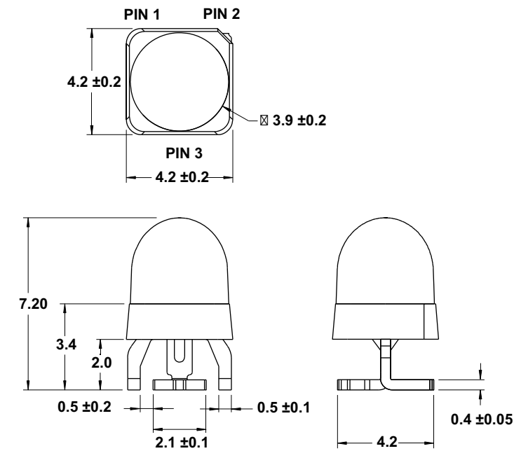
Figure 1: Package Drawing
