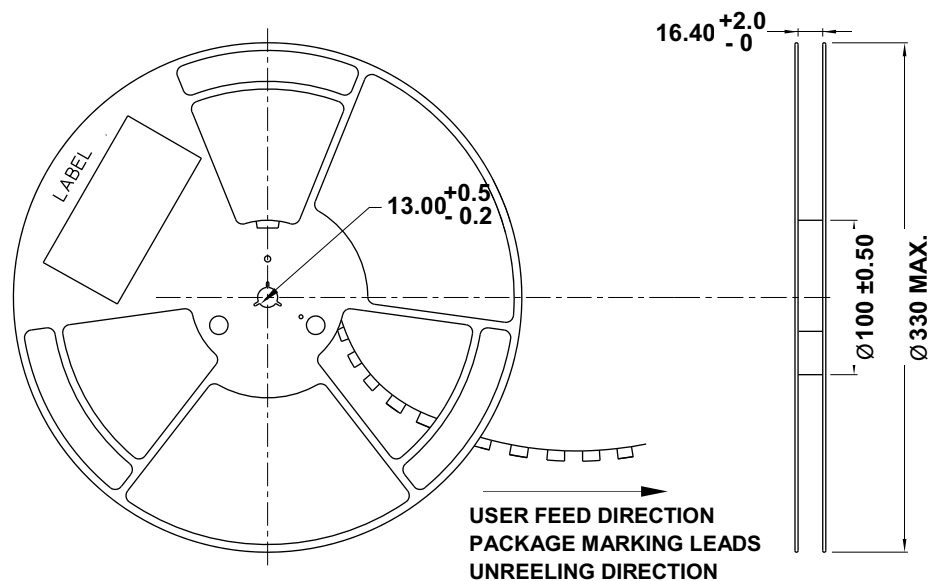
Figure 12: Reel Dimensions
