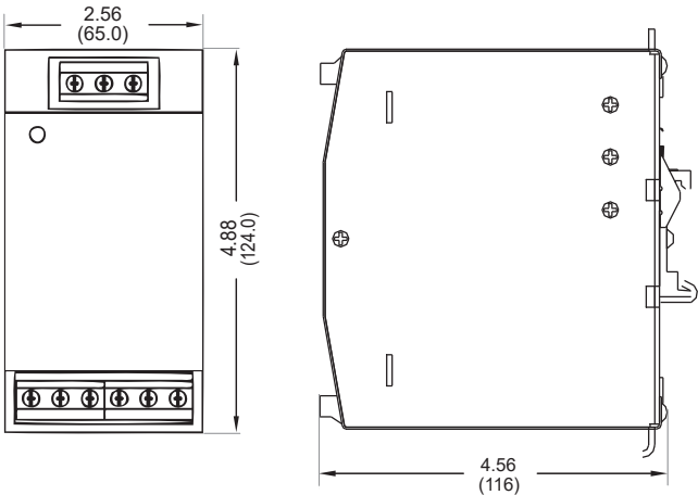
Dimensional Diagram - in. (mm)
