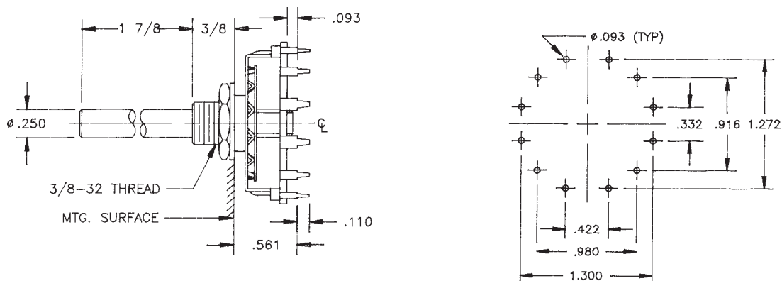
P.C. BOARD MOUNTING PATTERN
