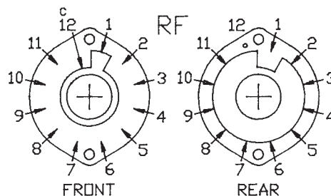
TWO POLE, 2-11 POSITION ALL UNUSED CLIPS CONNECTED AND SHORTED OUT
