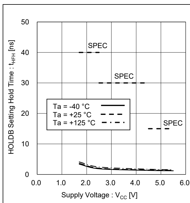
Figure 30. HOLDB Setting Hold Time vs Supply Voltage
