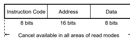
Figure 52. READ, RDID, RDLs Cancel Valid Timing
