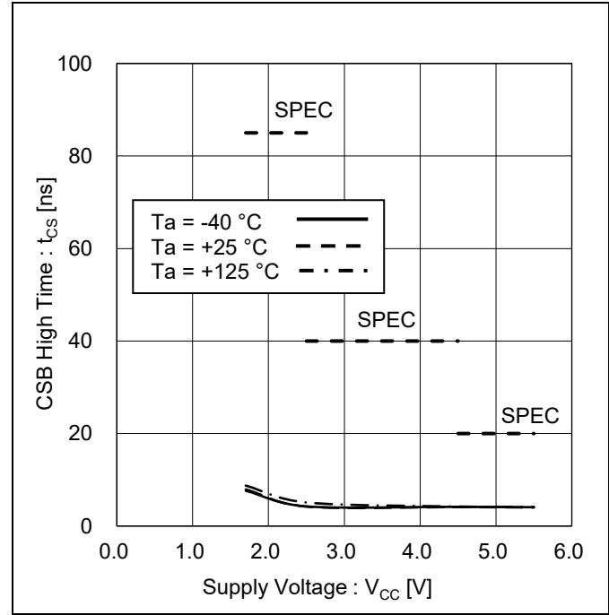
Figure 23. CSB High Time vs Supply Voltage
