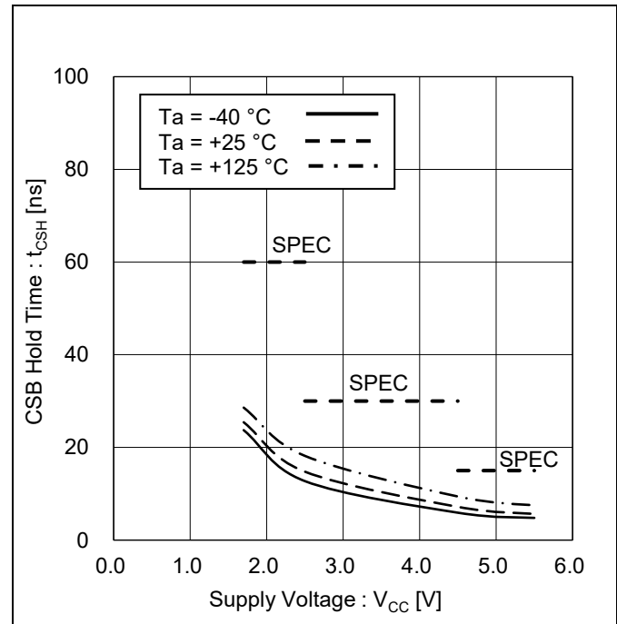
Figure 25. CSB Hold Time vs Supply Voltage
