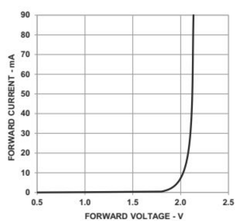
Figure 6: Forward Current vs. Forward Voltage
