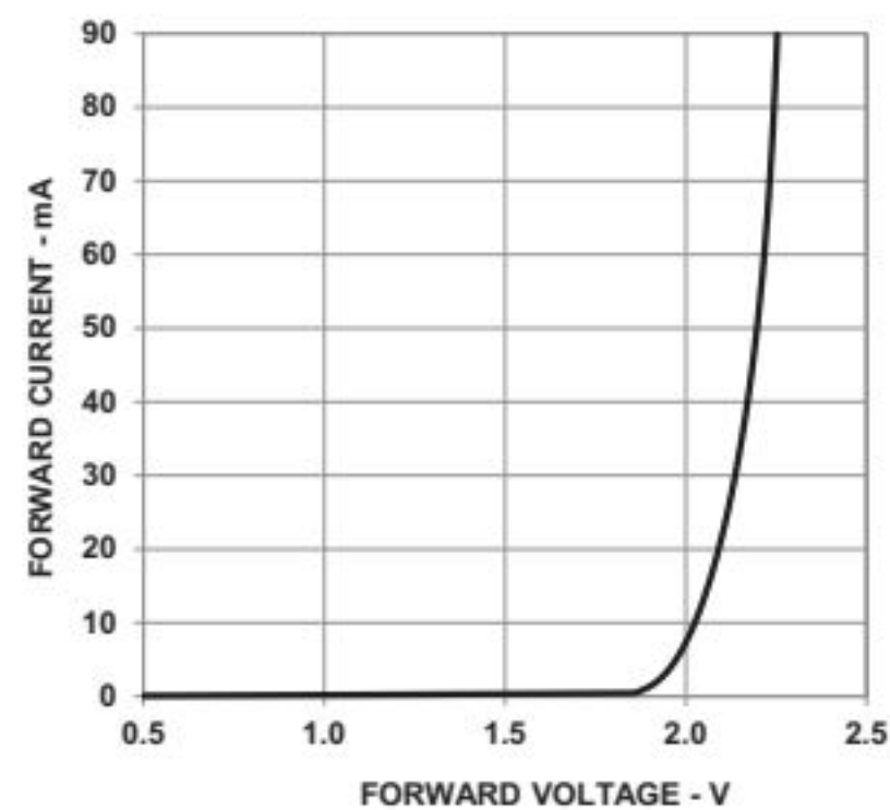
Figure 18: Forward Current vs. Forward Voltage
