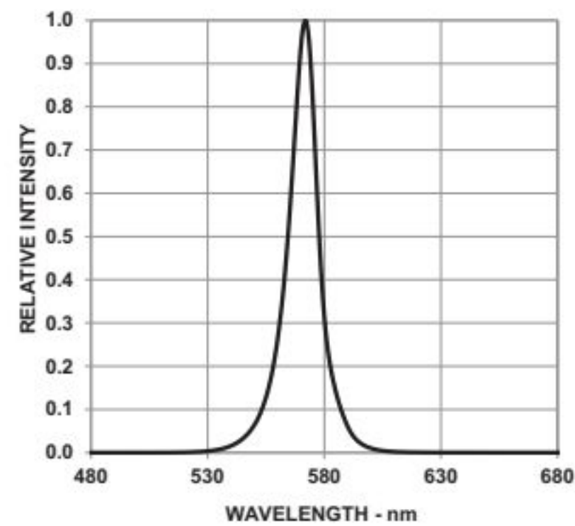
Figure 17: Relative Intensity vs. Wavelength
