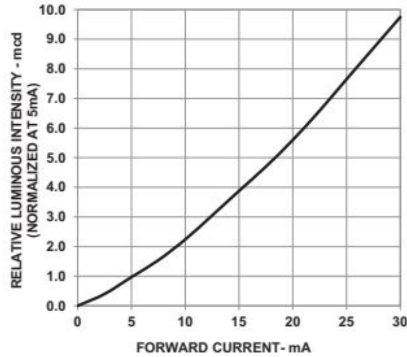
Figure 11: Relative Luminous Intensity vs. Forward Current
