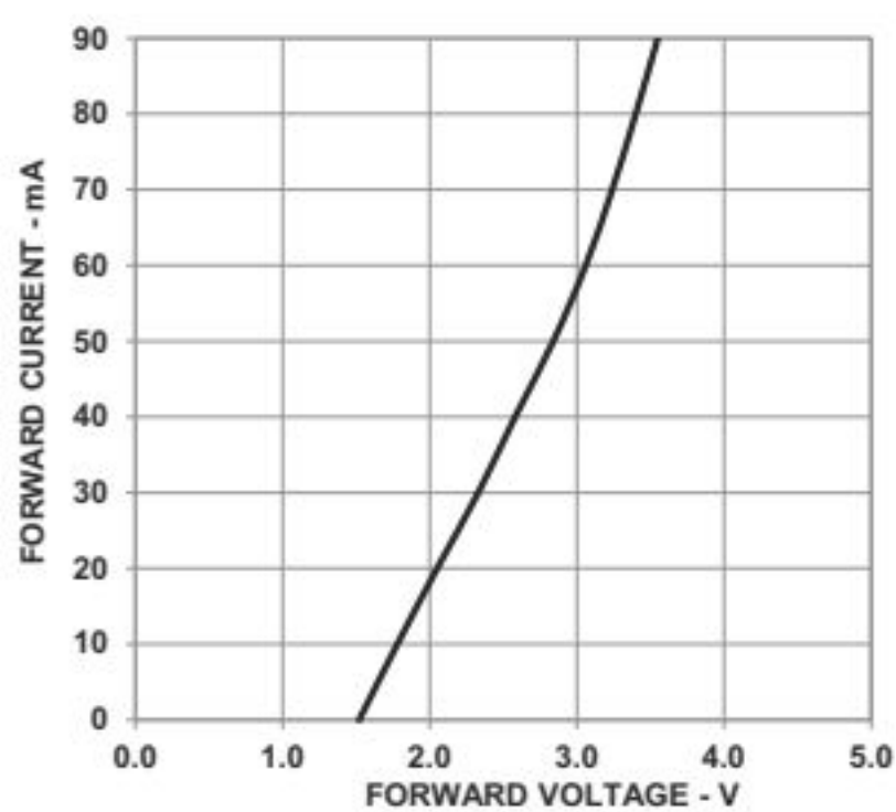
Figure 10: Forward Current vs. Forward Voltage
