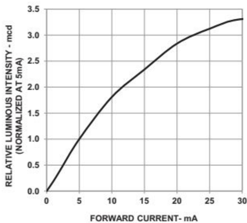
Figure 7: Relative Luminous Intensity vs. Forward Current
