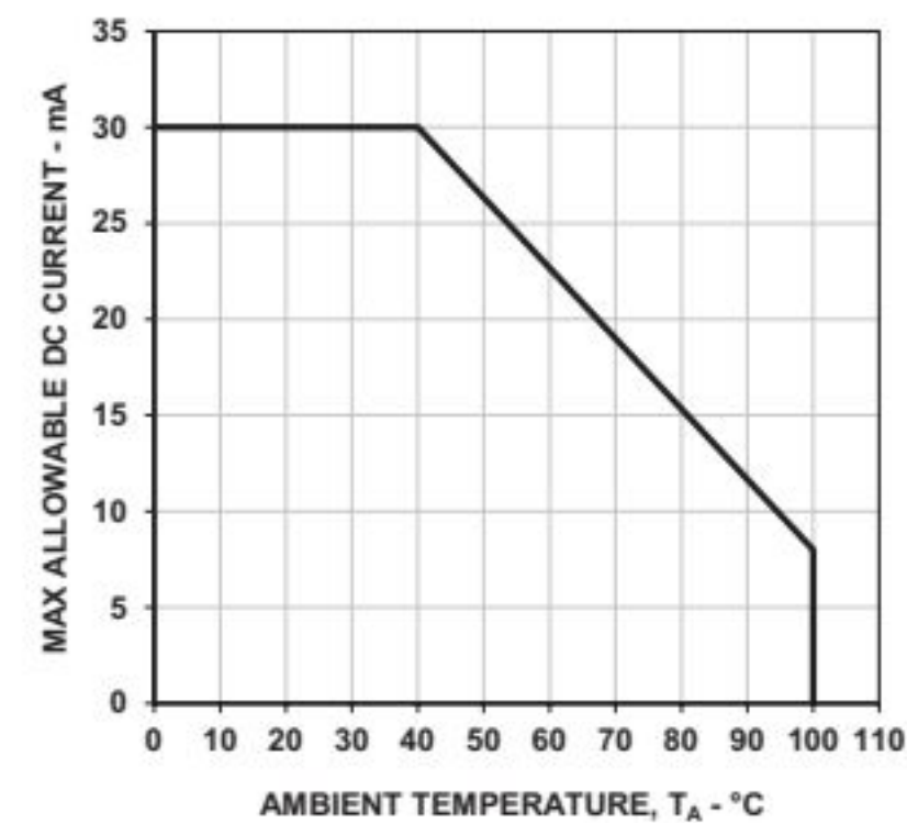
Figure 20: Maximum Forward Current vs. Ambient Temperature
