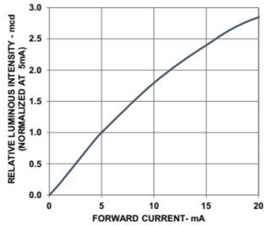
Figure 15: Relative Luminous Intensity vs. Forward Current
