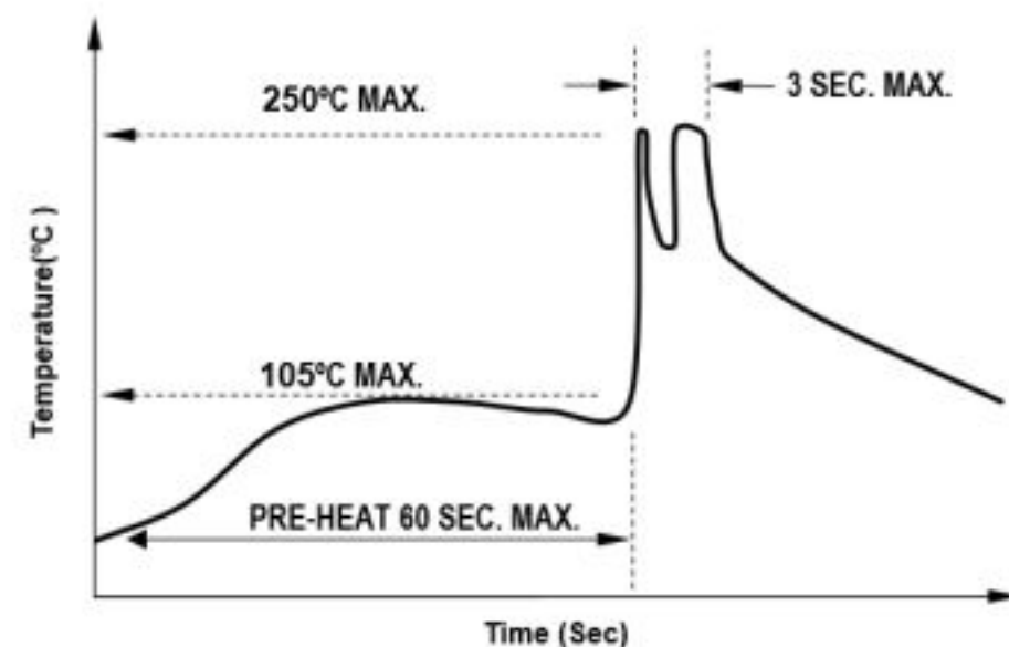
Figure 21: Recommended Wave Soldering Profile
