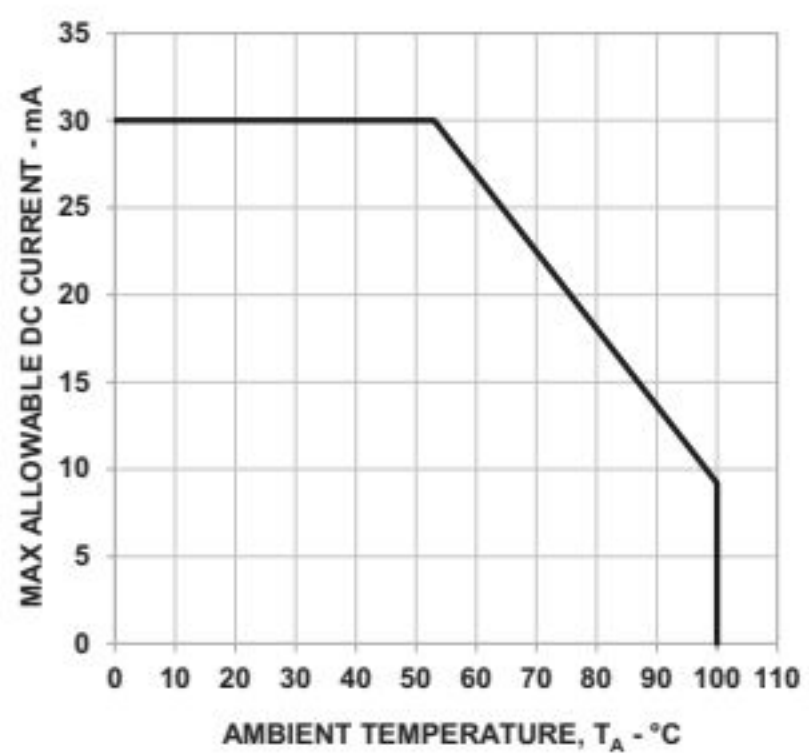
Figure 8: Maximum Forward Current vs. Ambient Temperature
