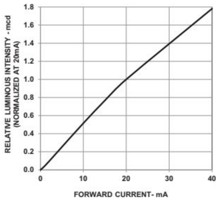
Figure 3: Relative Luminous Intensity vs. Forward Current
