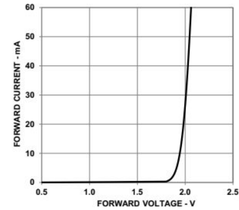
Figure 14: Forward Current vs. Forward Voltage
