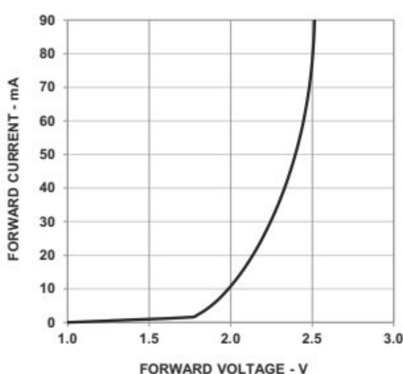
Figure 2: Forward Current vs. Forward Voltage
