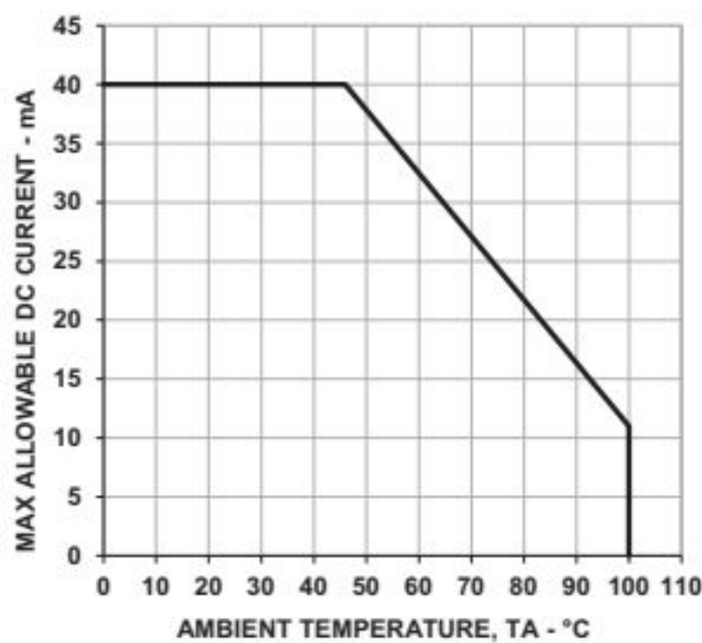
Figure 4: Maximum Forward Current vs. Ambient Temperature
