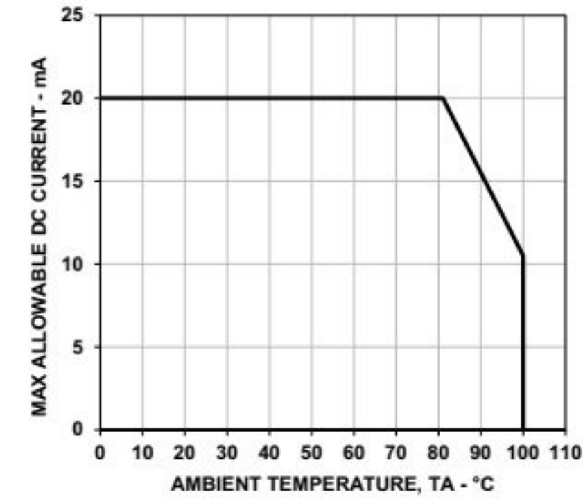
Figure 16: Maximum Forward Current vs. Ambient Temperature
