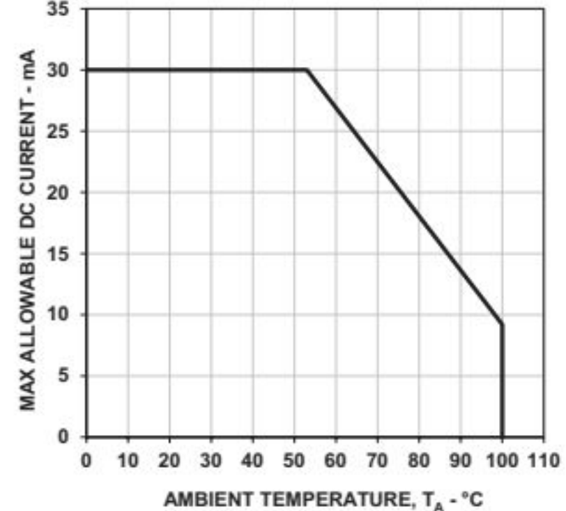
Figure 12: Maximum Forward Current vs. Ambient Temperature
