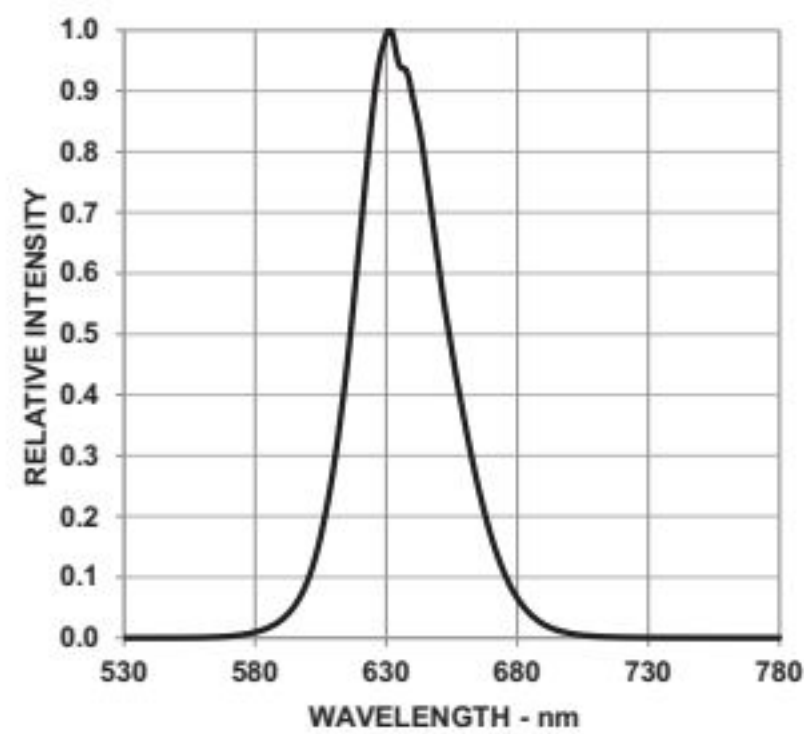
Figure 5: Relative Intensity vs. Wavelength
