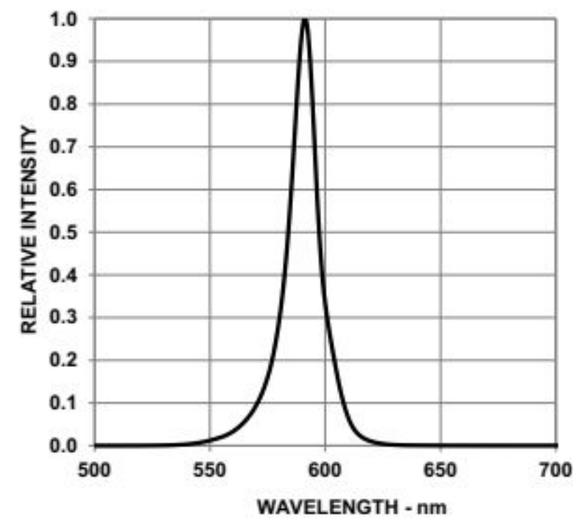
Figure 13: Relative Intensity vs. Wavelength
