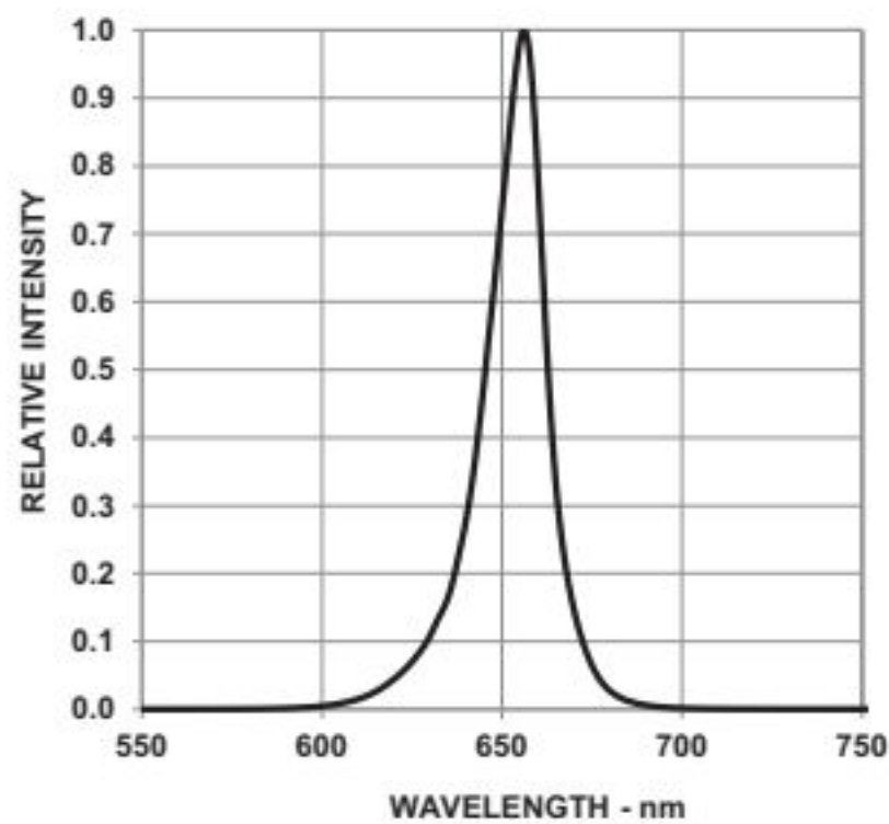
Figure 1: Relative Intensity vs. Wavelength
