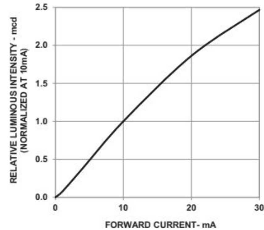
Figure 19: Relative Luminous Intensity vs. Forward Current
