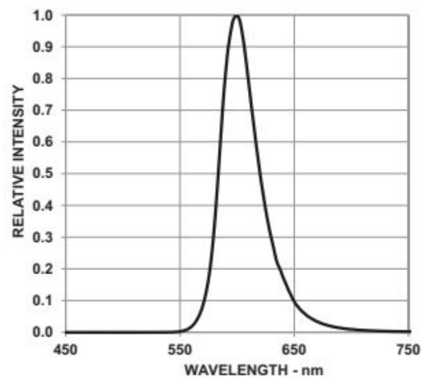
Figure 9: Relative Intensity vs. Wavelength
