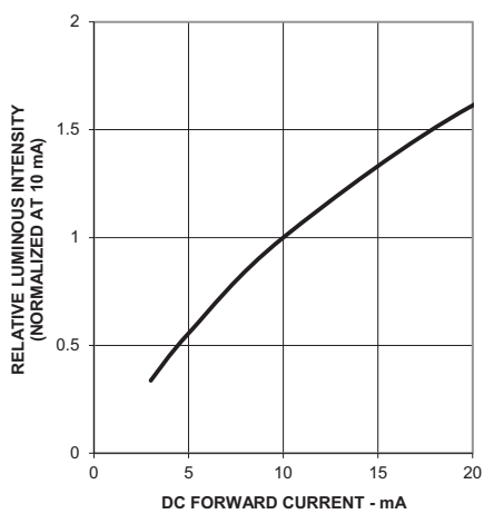
Figure 7: Relative Luminous Intensity vs. Forward Current
