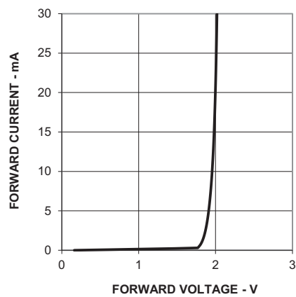
Figure 6: Forward Current vs. Forward Voltage Characteristics
