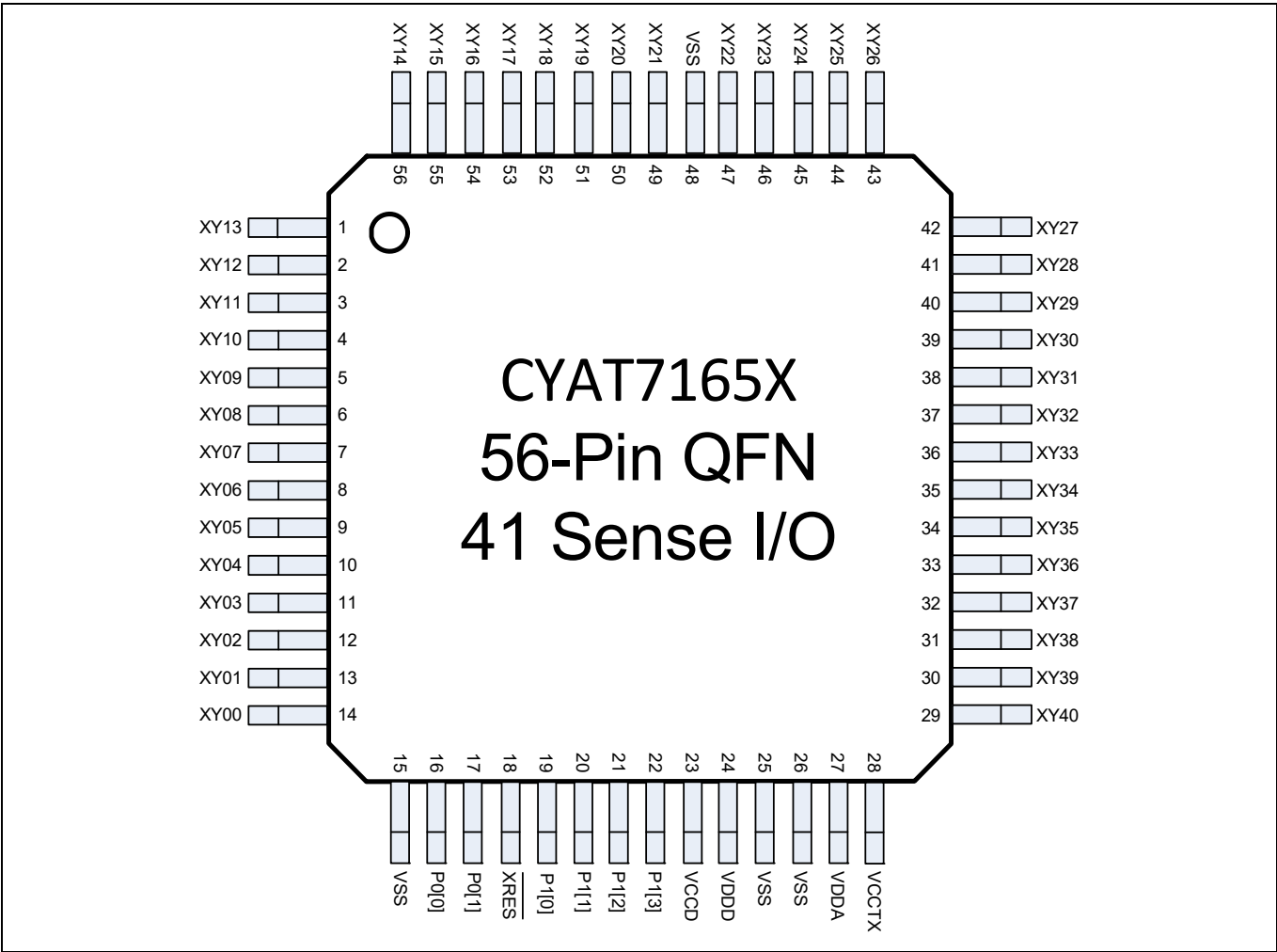
Figure 14 56-pin QFN pinout [10]
