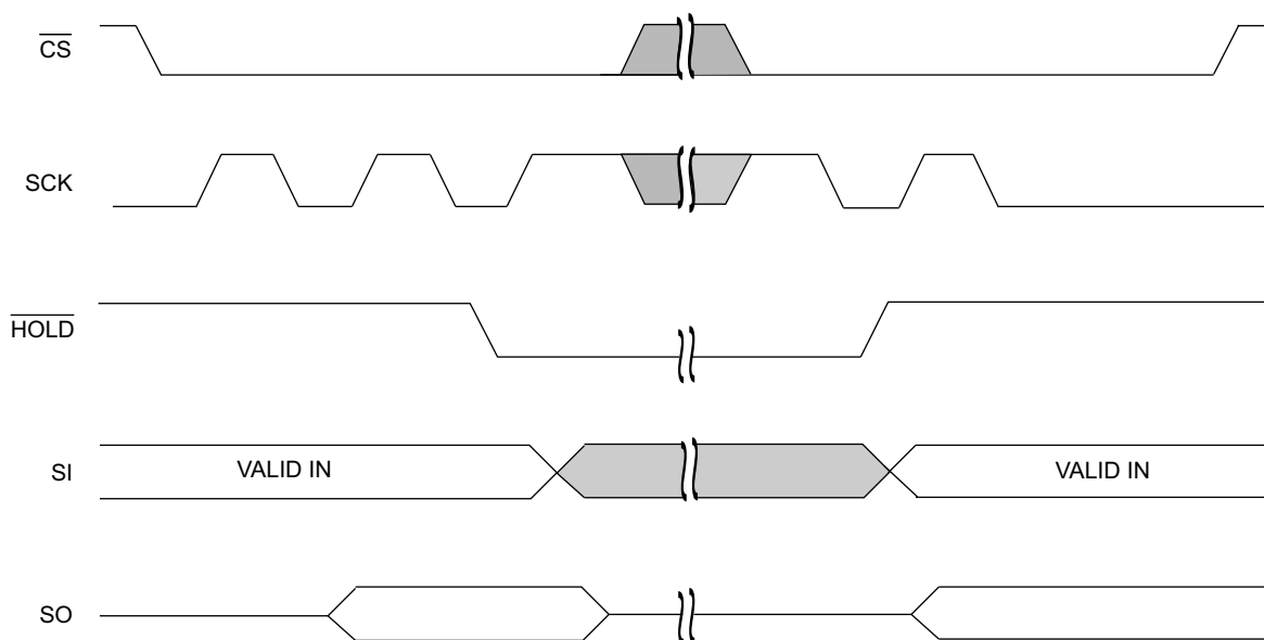
Figure 14. \overline{HOLD} Operation [2]
