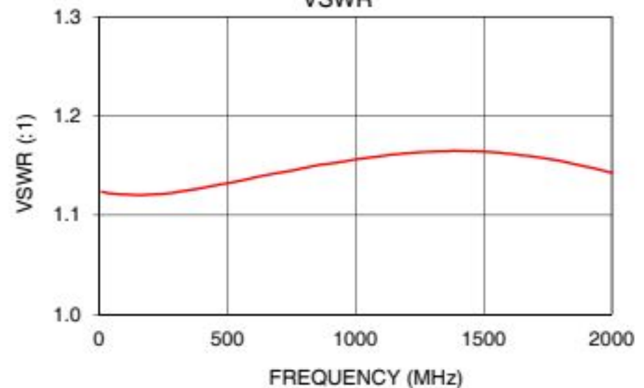
HAT-8A+ VSWR
