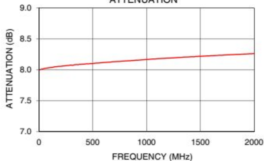
HAT-8A+ ATTENUATION
