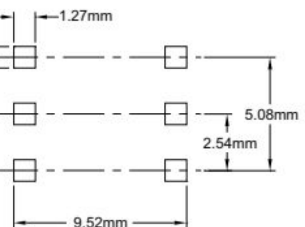
SUGGESTED PCB LAYOUT
