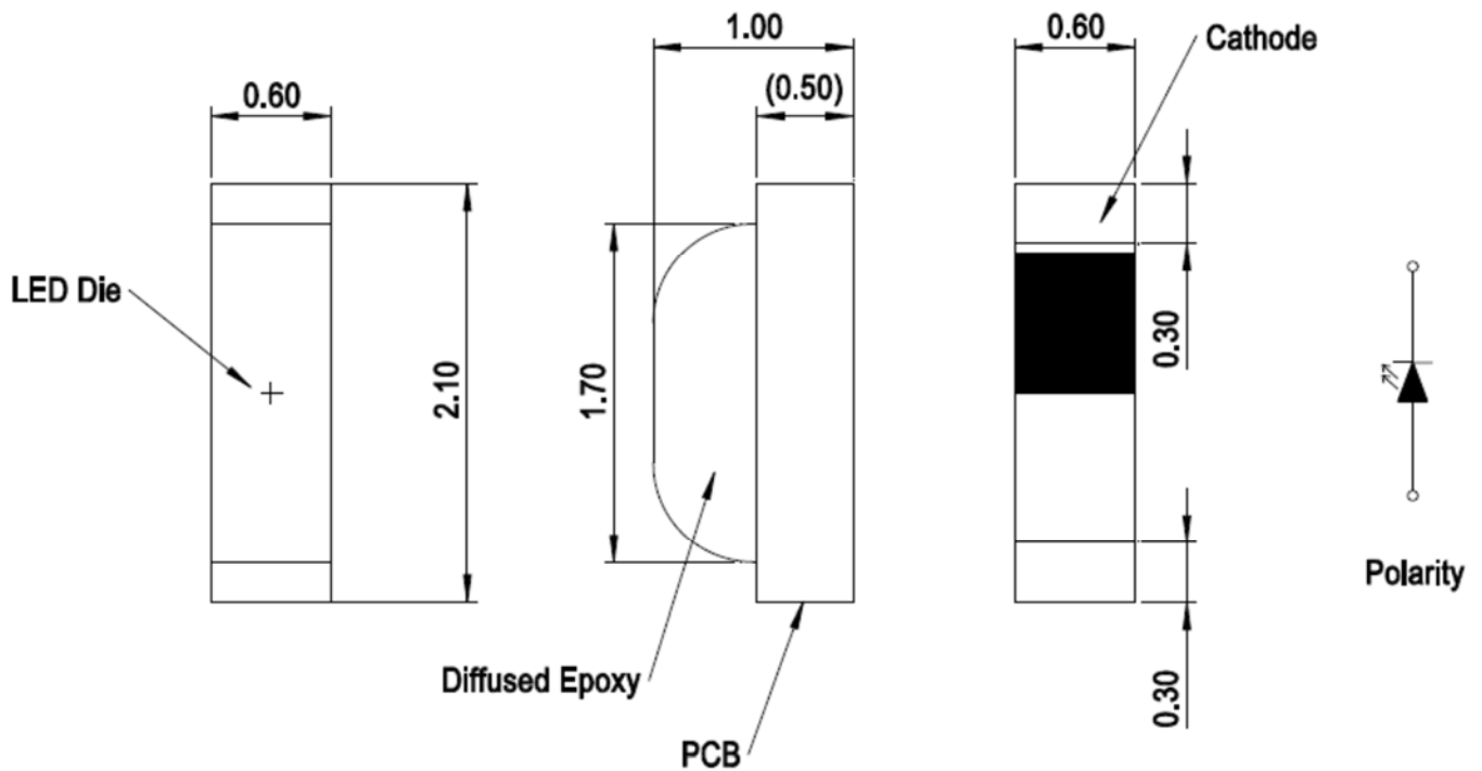
Figure 1: Package Dimensions
