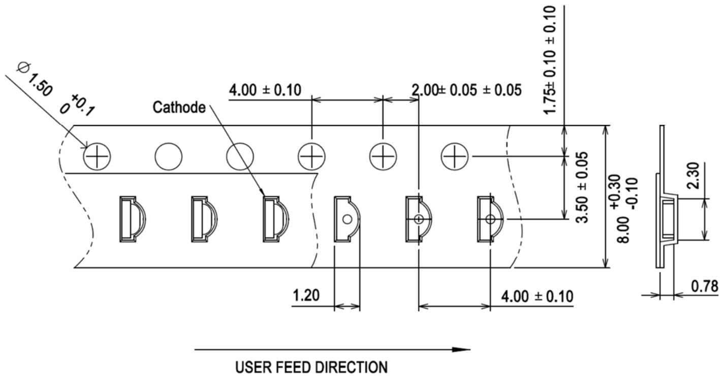
Figure 9: Carrier Tape Dimensions
