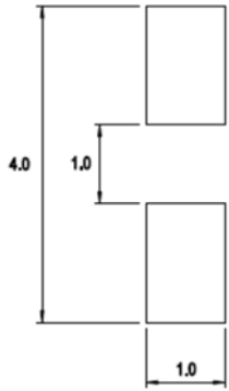
Figure 8: Recommended Soldering Land Pattern
