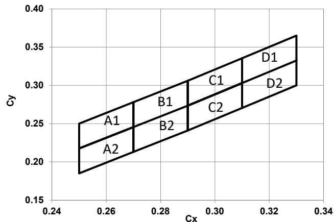
Figure 2: Chromaticity Diagram
