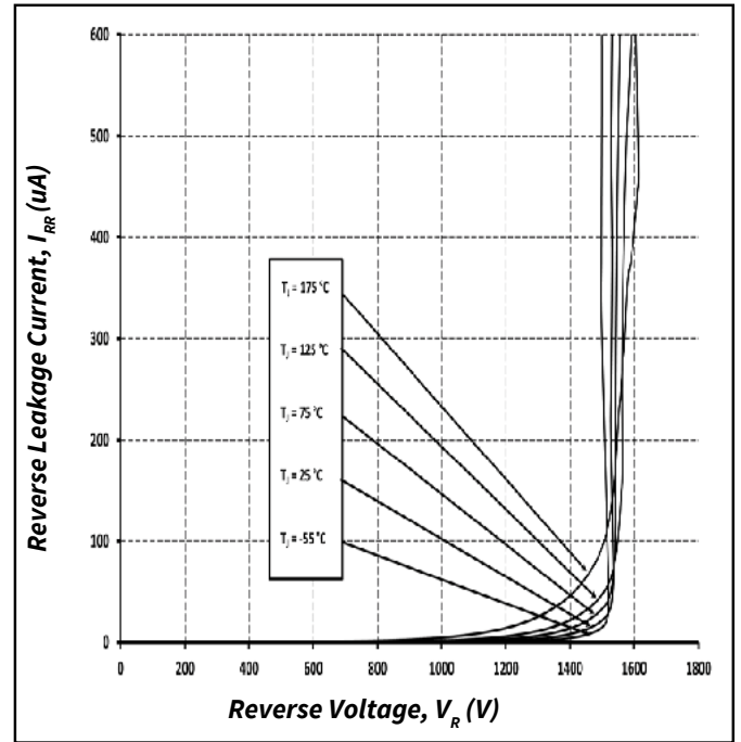
Figure 2. Reverse Characteristics
