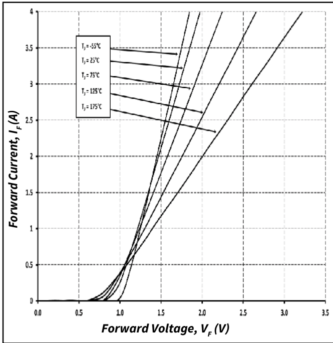
Figure 1. Forward Characteristics
