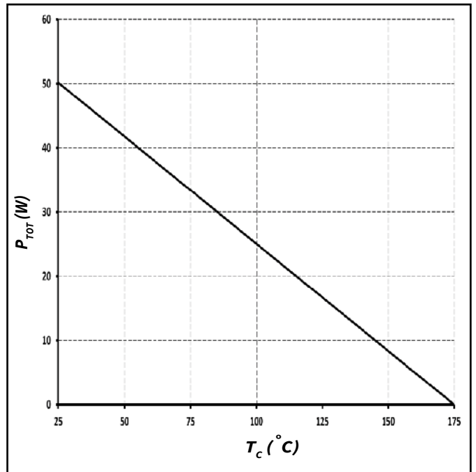
Figure 4. Power Derating
