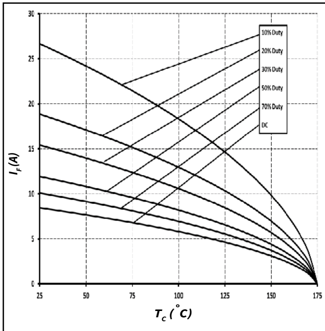
Figure 3. Current Derating
