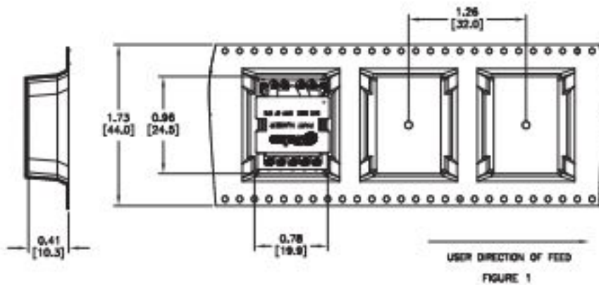
Tape & Reel Layout for PH08XXCNL
