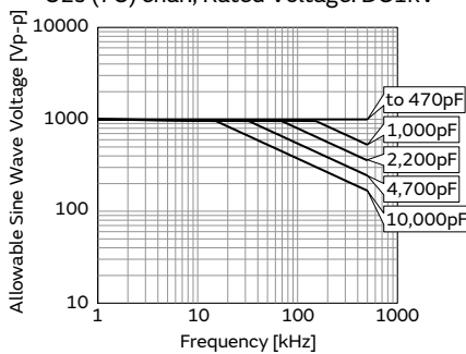
Chip (L×W): 3.2×1.6mm, 3.2×2.5mm 4.5×3.2mm, 5.7×5.0mm U2J (7U) char., Rated Voltage: DC1kV
