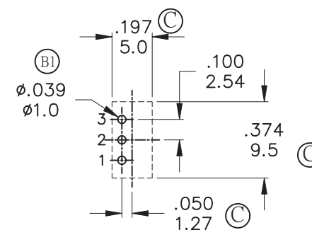
P.C. MOUNTING
