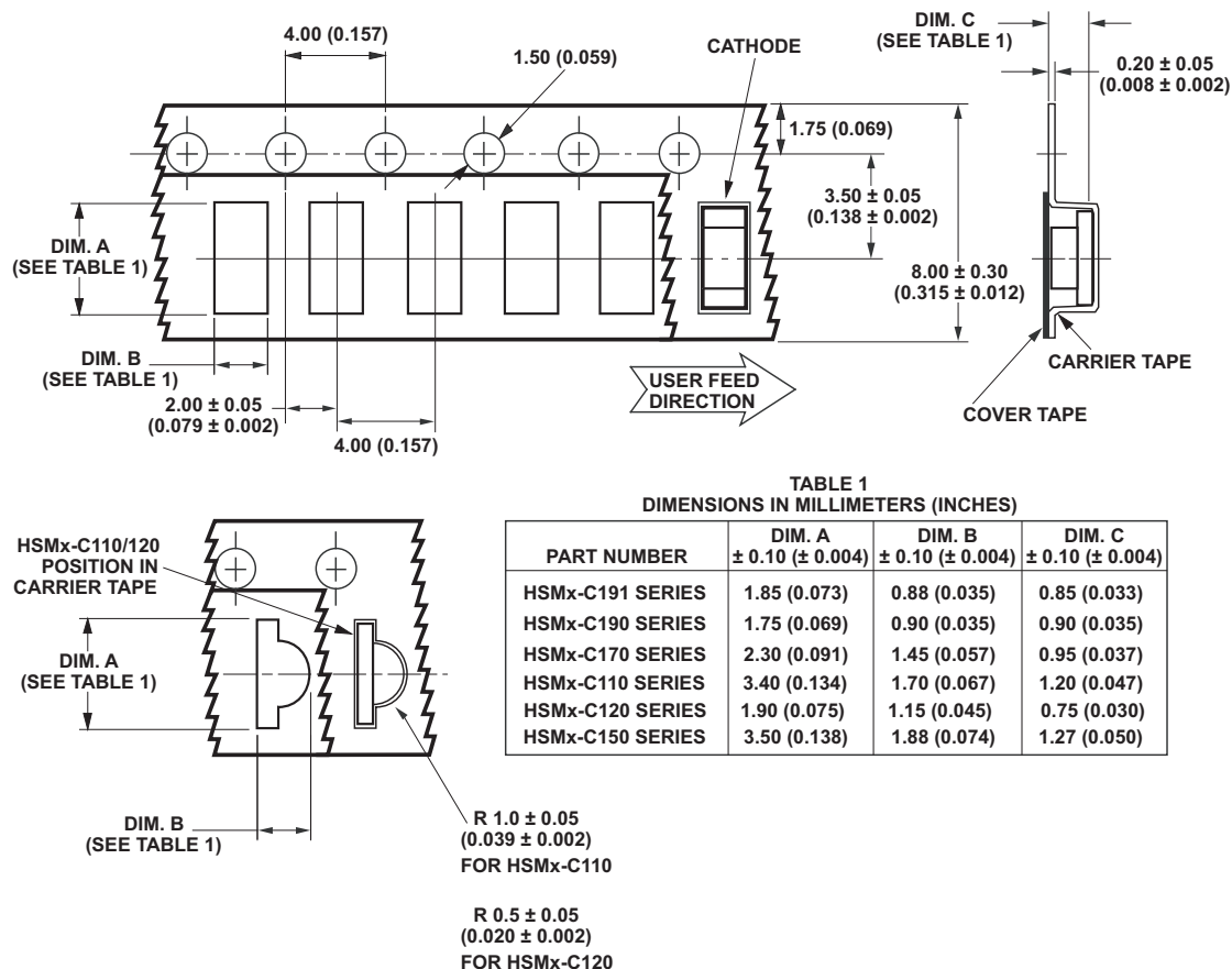
Figure 17. Tape dimensions.
