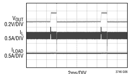
Adaptive LED Bus Voltage I
