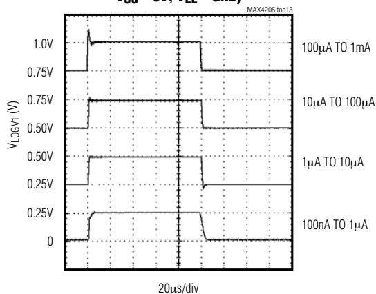
I_{REF} PULSE RESPONSE
