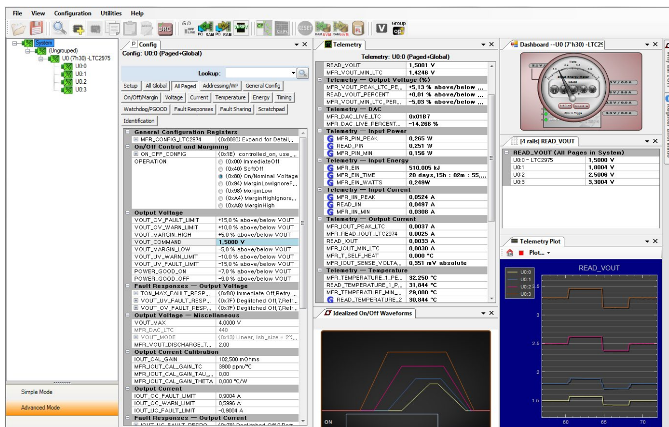
Figure 45. LTpowerPlay Snapshot
