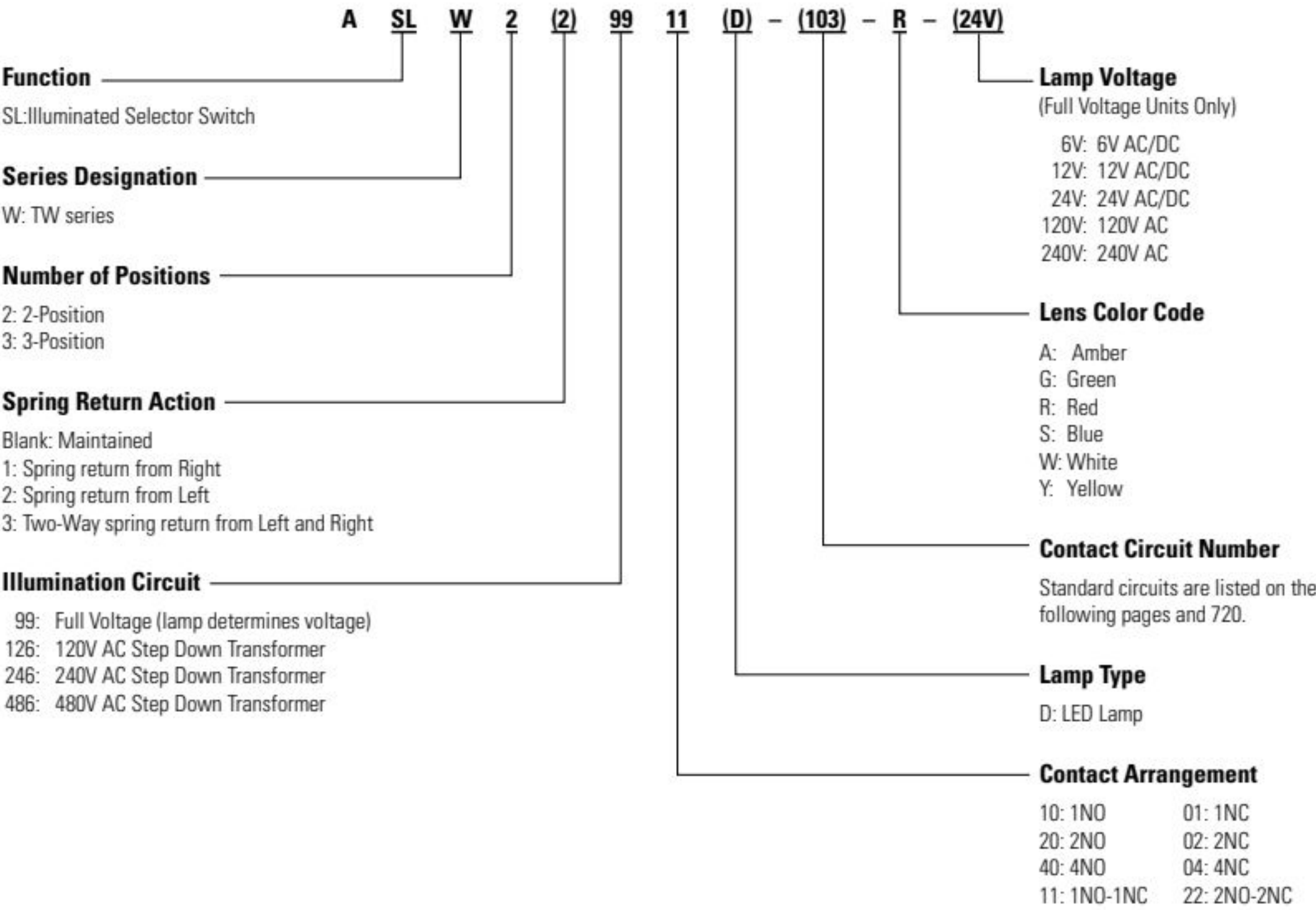
Assembled Illuminated Selector Switches
