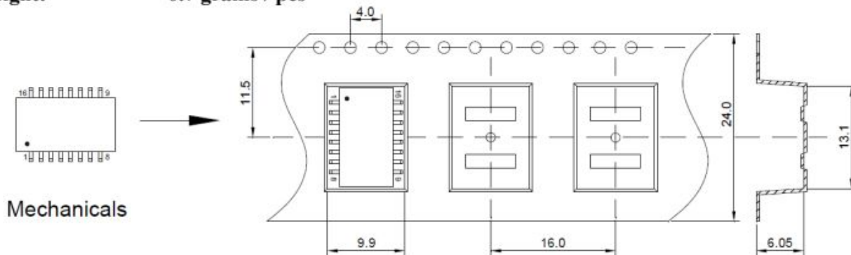
Tape & Reel
