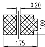
METAL MASK T=0.08
