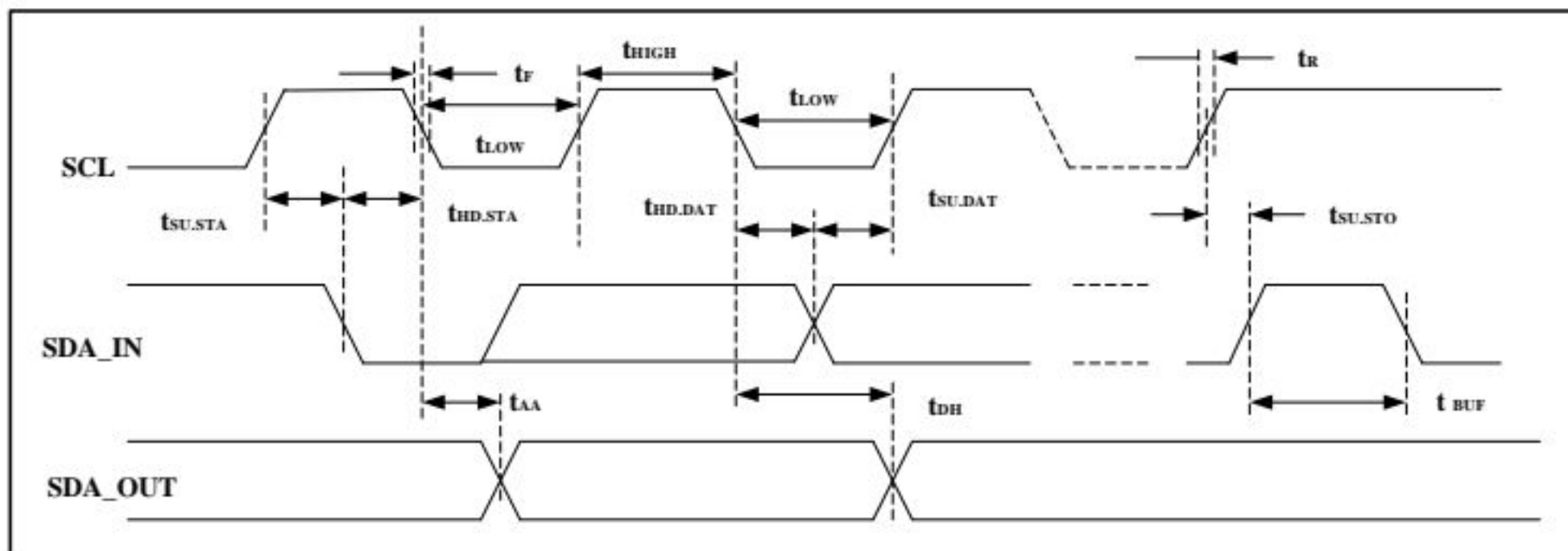
Figure 11. SCL: Serial Clock, SDA: Serial Data I/O
