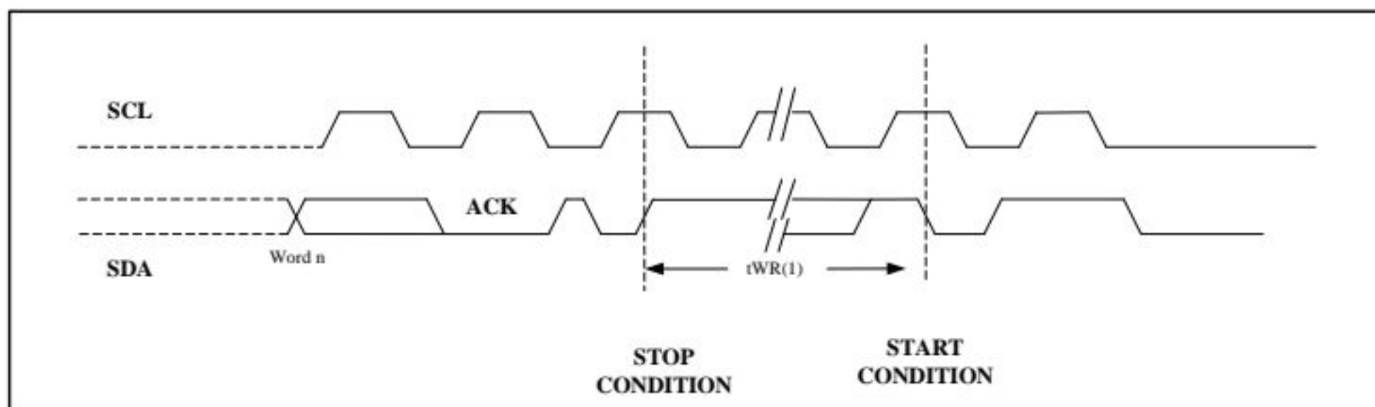
Figure 12. SCL: Serial Clock, SDA: Serial Data I/O
