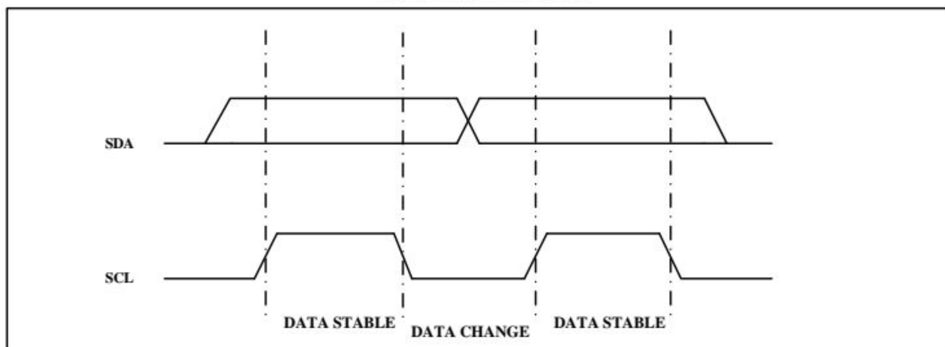
Figure 2. Data Validity
