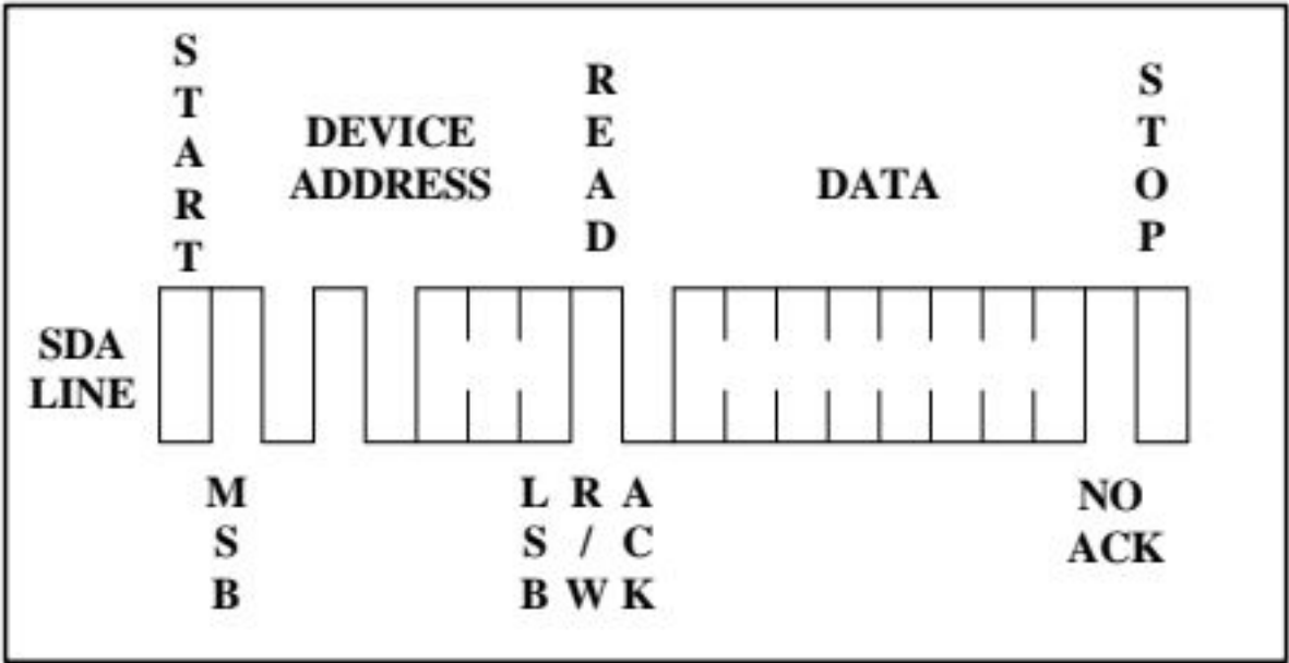
Figure 9. Random Read
