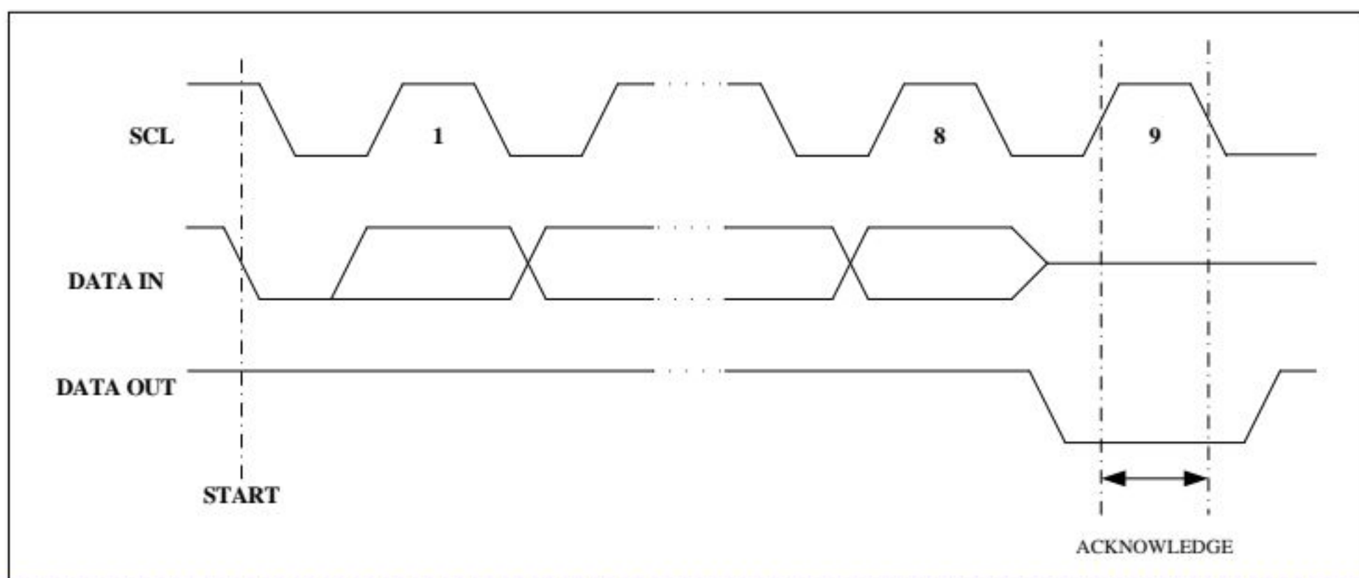
Figure 4. Output Acknowledge
