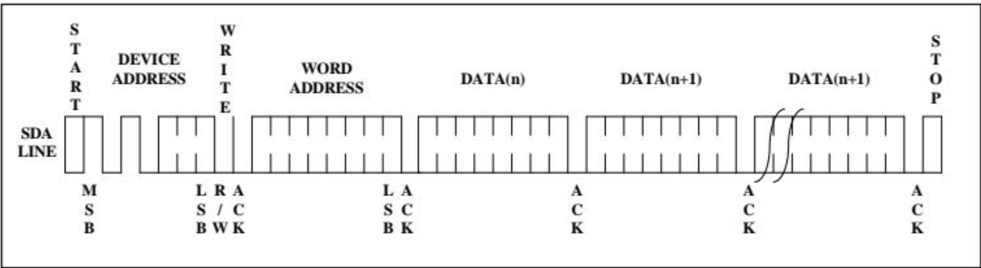
Figure 7. Page Write
