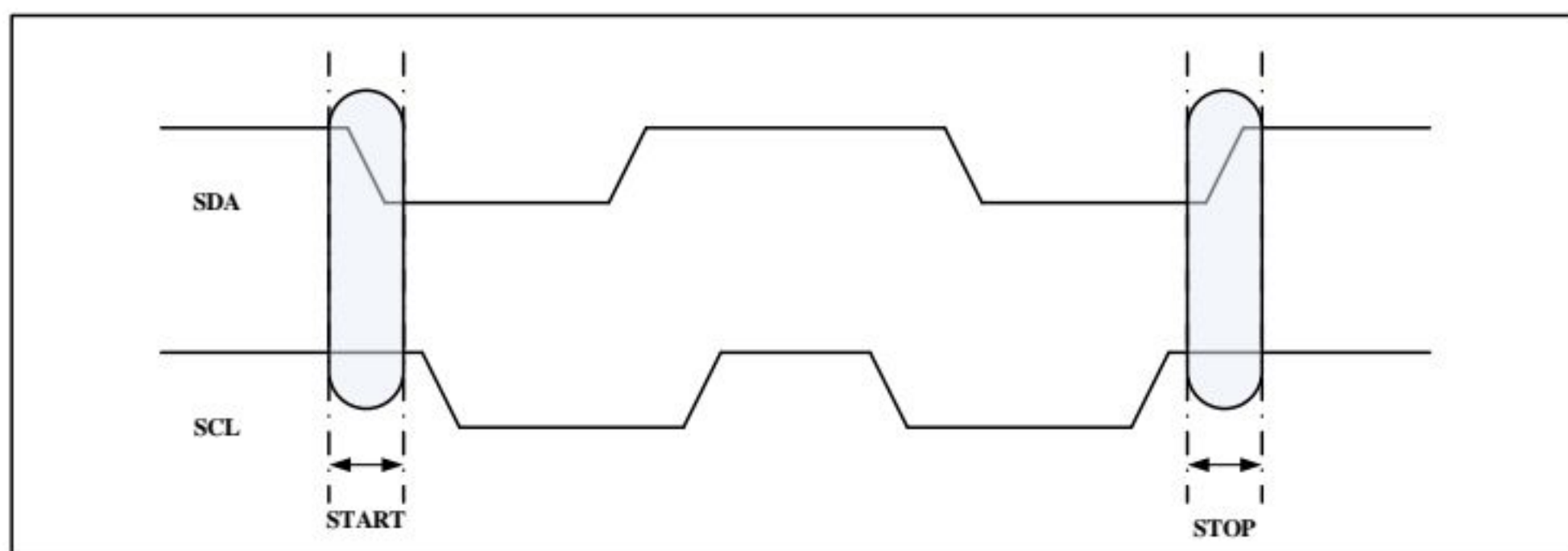
Figure 3. Start and Stop Definition
