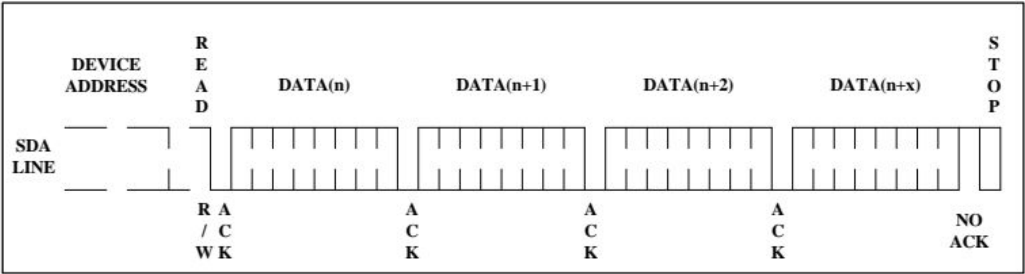
Figure 10. Sequential Read
